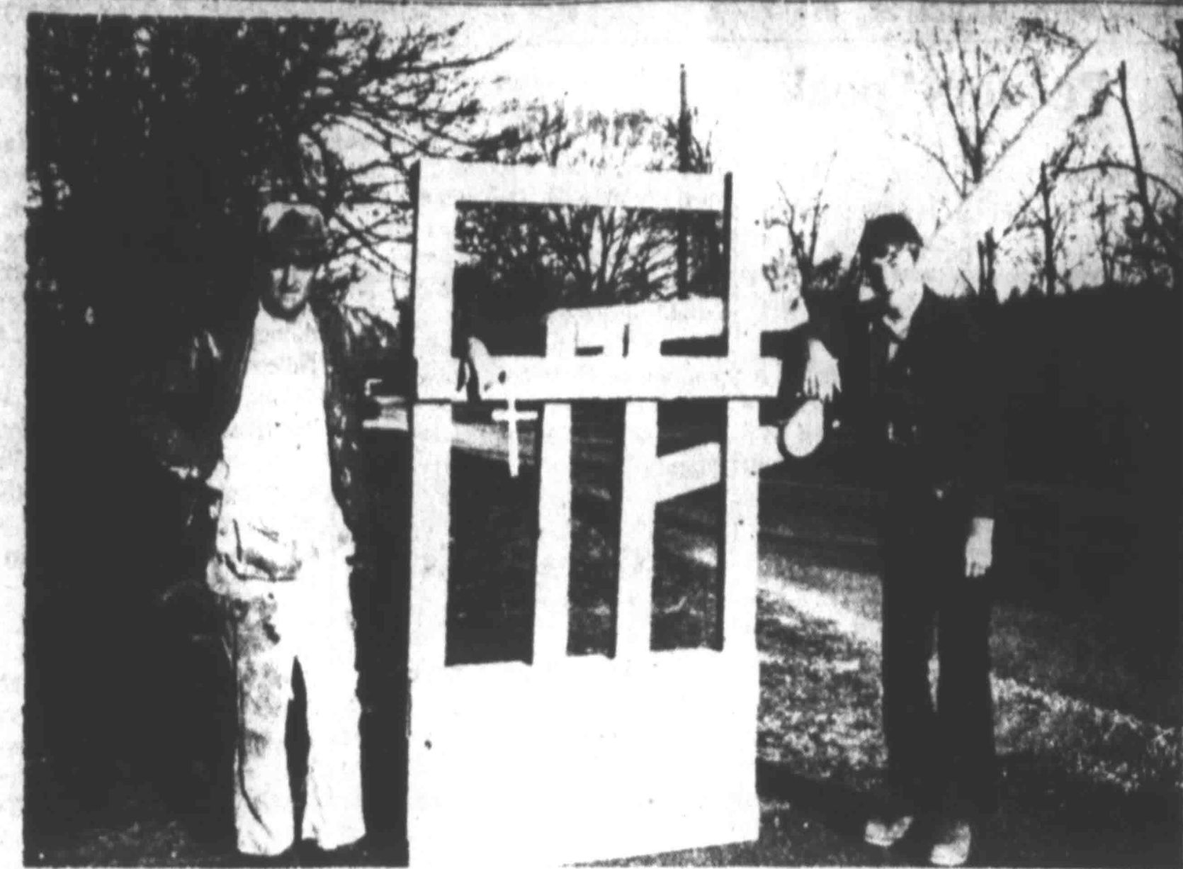
HEAD-GATE FOR HIS 4-H BEEF PROJECT was made by Gary Douglas (right), with the aid of Clyde Holder, of Curve (left), from cypress 2x4s and 1/2-inch carriage bolts, with a saw, square, drill, 3/4-inch bit, and wood rasp, following University of Tennessee Extension Service Head-Gates Plan 7241-13. A head-gate facilitates handling cattle when they are being vaccinated, de-horned, branded, ear-tagged, or treated for disease or parasites. Commercially constructed ones may cost $100 or more, but one can be built with about $25 worth of materials. Plans for such head-gates, and for many other types of livestock equipment and buildings, will be mailed to persons requesting them by phoning 635-9551.
